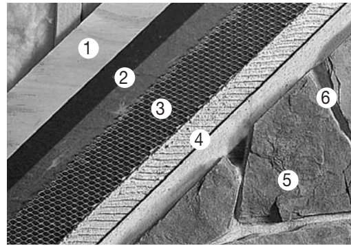
In sequence: (1) sheathing, (2) two layers of water resistant barrier, (3) galvanized metal lath, (4) mortar/scratch coat/setting bed (5) Cultured Stone ® manufactured stone veneer, (6) mortar joint.
