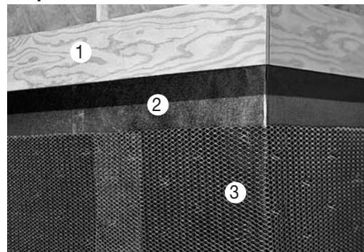
Water resistant barrier and lath must continuously wrap a minimum of 16” at outside and inside corners and fasten at a framing member. Lap water resistant barrier a minimum of 4” at vertical and 2” at horizontal lap joints. Lap lath a minimum of 1” at vertical and horizontal seams. (1) wall substrate, (2) two layers of water resistant barrier, (3) metal lath.
