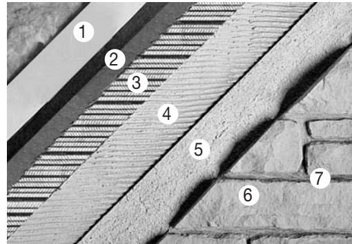
In sequence: (1) rigid foam insulation, (2) two layers of water resistant barrier, (3) galvanized metal lath, (4) scratch coat, (5) mortar setting bed, (6) Cultured Stone ® manufactured stone veneer, (7) mortar joint.
