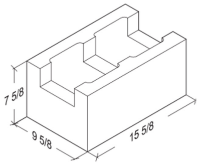
10-8-16 Bond Beam 9 5/8" x 7 5/8" x 15 5/8"
