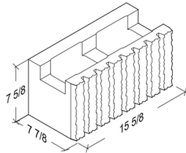
8-8-16 7-Score Bond Beam 7 5/8" x 7 7/8" x 15 5/8"
