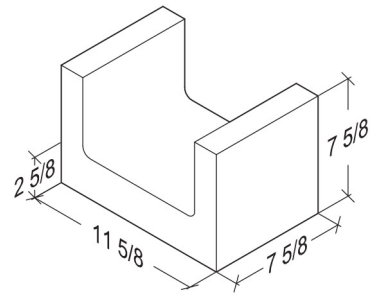
12-8-8 Lintel 11 5/8" x 7 5/8" x 7 5/8"
