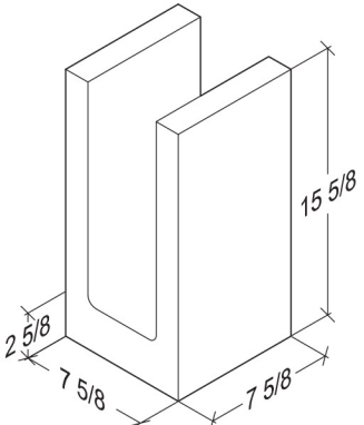
8-8-16 Lintel 7 5/8" x 7 5/8" x 15 5/8"
