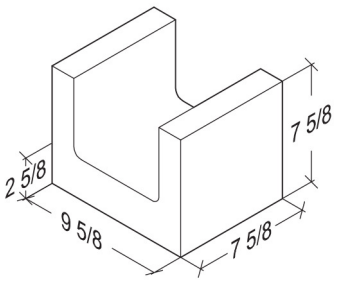
10-8-8 Lintel 9 5/8" x 7 5/8" x 7 5/8"
