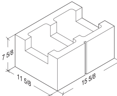
12-8-16 1-Score Bond Beam 11 5/8" x 7 5/8" x 15 5/8"
