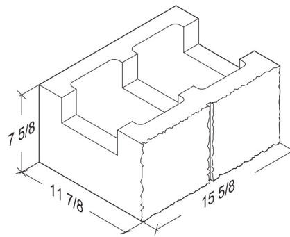
12-8-16 1-Score Bond Beam
