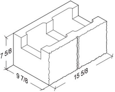
10-8-16 1-Score Bond Beam 9 7/8" x 7 5/8" x 15 5/8"
