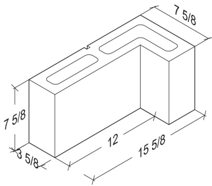
4 Inch L-Corner
