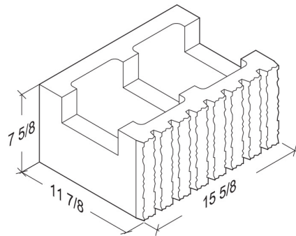
12-8-16 7-Score Bond Beam
