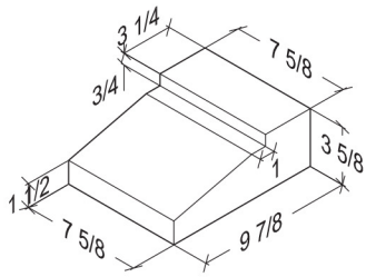
10x4x8 Square Sill
