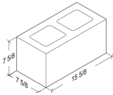
8-8-16 Standard 7 5/8" x 7 5/8" x 15 5/8"
