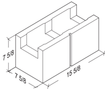
8-8-16 1-Score Bond Beam 7 5/8" x 7 5/8" x 15 5/8"
