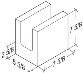
6-8-8 Lintel 5 5/8" x 7 5/8" x 7 5/8"
