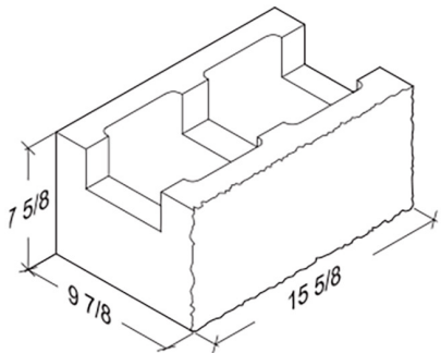
10-8-16 Bond Beam 9 7/8" x 7 5/8" x 15 5/8"
