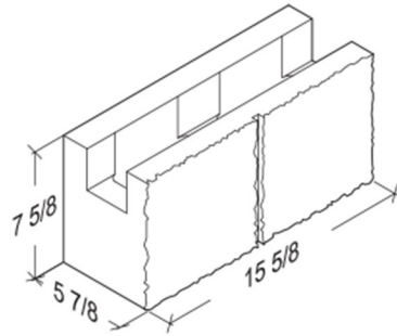
6-8-16 1-Score Bond Beam 5 5/8" x 7 5/8" x 15 5/8"
