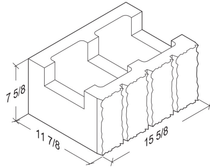
12-8-16 3-Score Bond Beam
