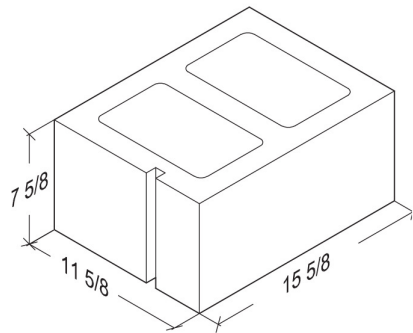
12-8-16 Standard 11 5/8" x 7 5/8" x 15 5/8"
