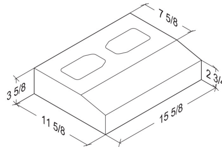
12x4x16 Square Transition Sill
