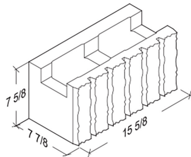
8-8-16 5-Score Bond Beam 7 5/8" x 7 7/8" x 15 5/8"
