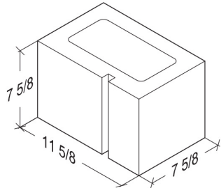
12-8-8 Half 11 5/8" x 7 5/8" x 7 5/8"
