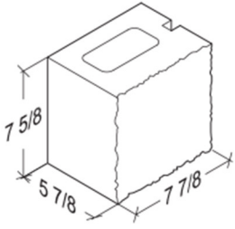
6-8-8 Half 5 5/8" x 7 5/8" x 7 7/8"
