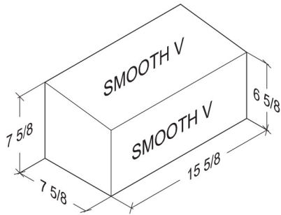
8x8x16 Sloped Sill
