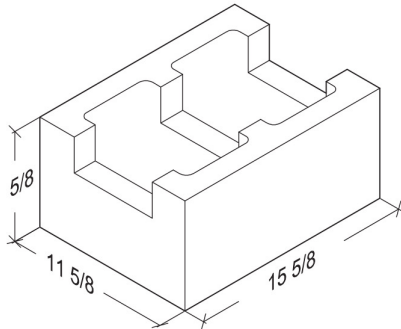
12-8-16 Bond Beam 11 5/8" x 7 5/8" x 15 5/8"
