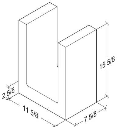
12-8-16 Lintel 11 5/8" x 7 5/8" x 15 5/8"
