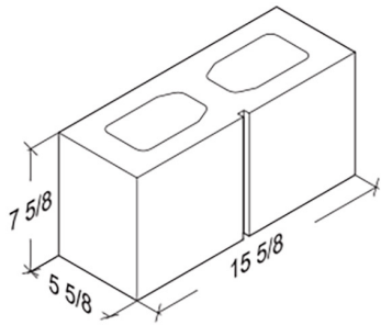
6-8-16 1-Score 5 5/8" x 7 5/8" x 15 5/8"
