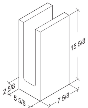
6-8-16 Lintel 5 5/8" x 7 5/8" x 15 5/8"
