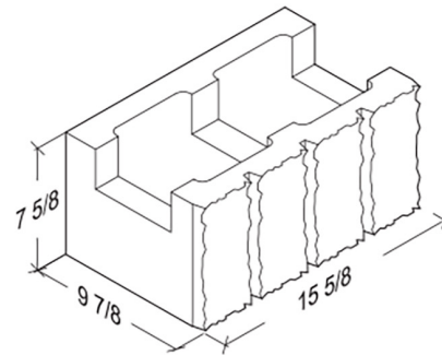
10-8-16 3-Score Bond Beam 9 7/8" x 7 5/8" x 15 5/8"
