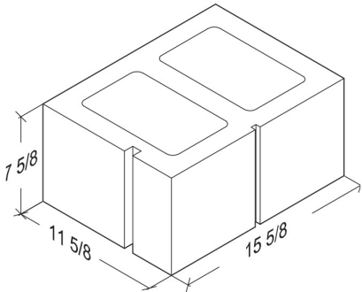
12-8-16 1-Score 11 5/8" x 7 5/8" x 15 5/8"
