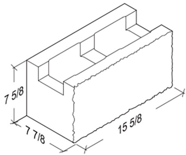
8-8-16 Bond Beam 7 5/8" x 7 7/8" x 15 5/8"
