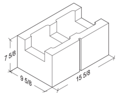
10-8-16 1-Score Bond Beam 9 5/8" x 7 5/8" x 15 5/8"
