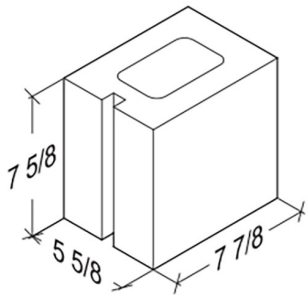
6-8-8 Half 5 5/8" x 7 5/8" x 7 7/8"
