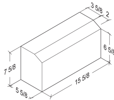
6x8x16 Chamfer B
