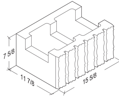
12-8-16 5-Score Bond Beam
