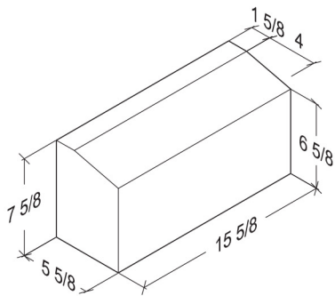
6x8x16 - Chamfer A
