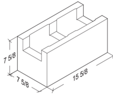
8-8-16 Bond Beam 7 5/8" x 7 5/8" x 15 5/8"
