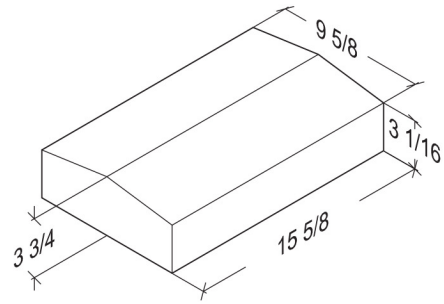
10-4-16 Sloped Cap 9 5/8" x 3 3/4" x 15 5/8"
