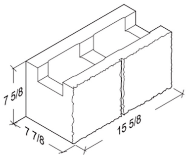
8-8-16 1-Score Bond Beam 7 5/8" x 7 7/8" x 15 5/8"
