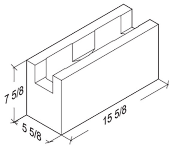
6-8-16 Bond Beam 5 5/8" x 7 5/8" x 15 5/8"
