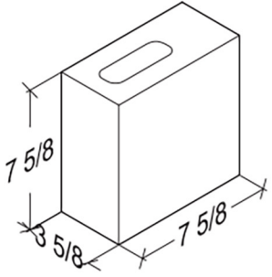
4-8-8 Half 3 5/8" x 7 5/8" x 7 5/8"
