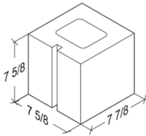
8-8-8 Half 7 5/8" x 7 5/8" x 7 7/8"
