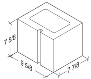
10-8-8 Half 9 5/8" x 7 5/8" x 15 5/8"
