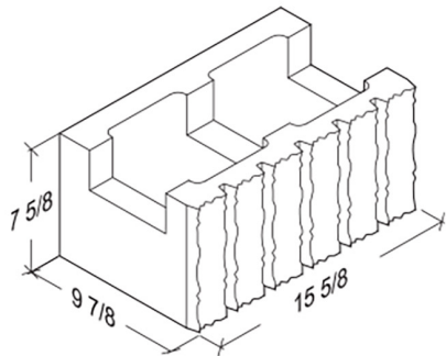
10-8-16 5-Score Bond Beam 9 7/8" x 7 5/8" x 15 5/8"
