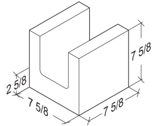
8-8-8 Lintel 7 5/8" x 7 5/8" x 7 5/8"
