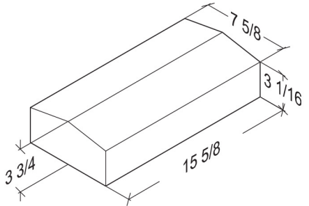
8-4-16 Sloped Cap 7 5/8" x 3 3/4" x 15 5/8"
