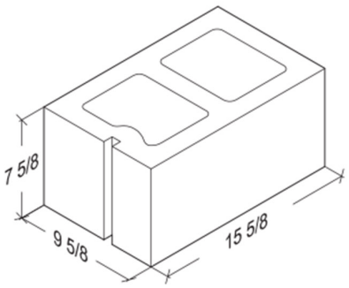
10-8-16 Standard 9 5/8" x 7 5/8" x 15 5/8"
