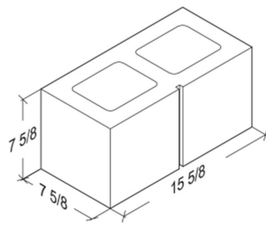
8-8-16 1-Score 7 5/8" x 7 5/8" x 15 5/8"
