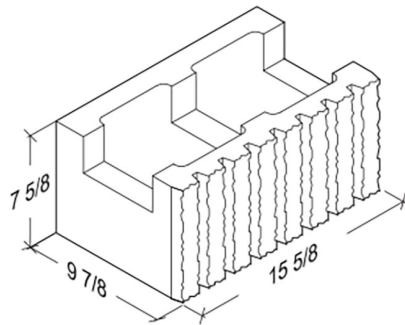
10-8-16 7-Score Bond Beam 9 7/8" x 7 5/8" x 15 5/8"
