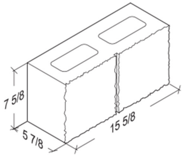
6-8-16 1-Score 5 5/8" x 7 5/8" x 15 5/8"
