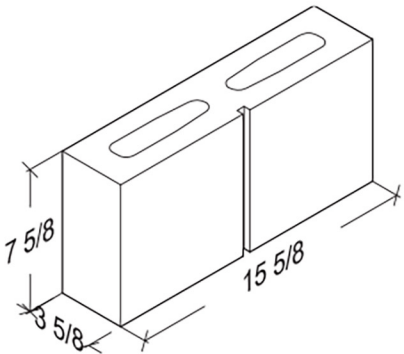
4-8-16 1-Score 3 5/8" x 7 5/8" x 15 5/8"
