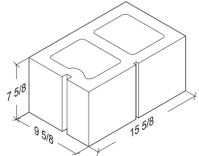
10-8-16 1-Score 9 5/8" x 7 5/8" x 15 5/8"
