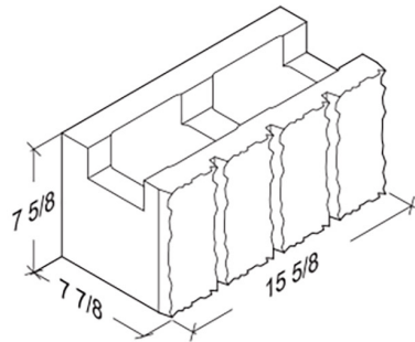
8-8-16 3-Score Bond Beam 7 5/8" x 7 7/8" x 15 5/8"
