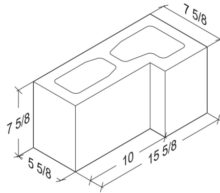
6 Inch L-Corner
